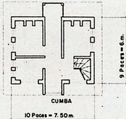
FIRST FLOOR PLAN BİRİNCİ KAT PLANI
