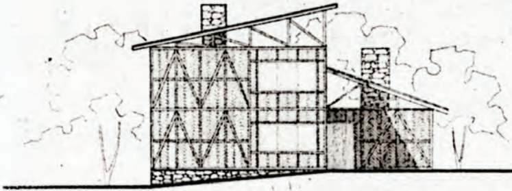
REAR ELEVATION ARKA CEPHE
