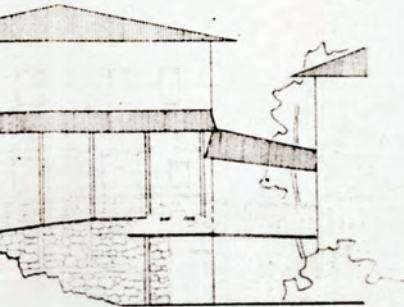
SOUTH ELEVATION GÜNEY CEPHESİ
