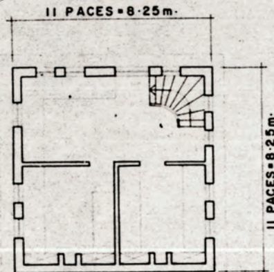
FIRST FLOOR PLAN BİRİNCİ KAT PLANI
